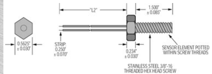
H7229 Hex Bolt, 3/8"-16 Thread, High Temperature
